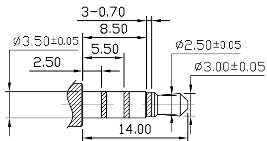
(ø3.50mm 4 POLE PLUG DETAIL DRAWING)
