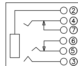
CIRCUIT
