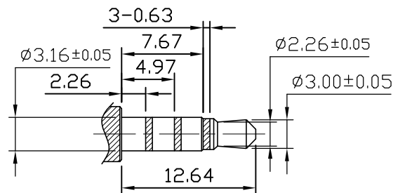
(ø3.50mm 4 POLE PLUG DETAIL DRAWING)
