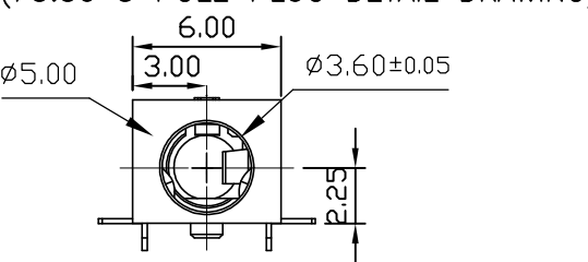
(Ø3.50 3 POLE PLUG DETAIL DRAWING)
