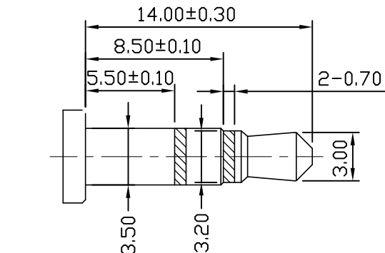
(Ø3.50 3 POLE PLUG DETAIL DRAWING)
