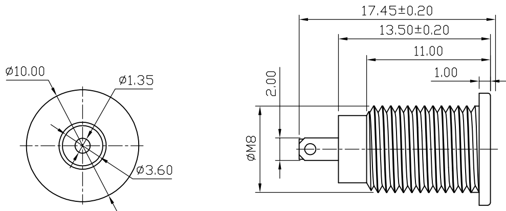
螺帽
