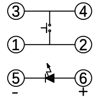
CIRCUIT
